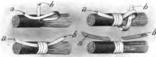
FIG. 105b.—Cable forming.
